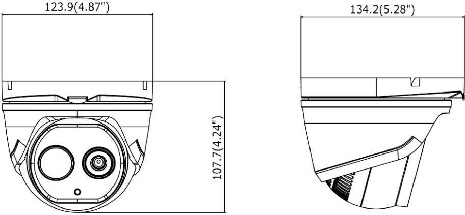
Unit: mm(inch)
